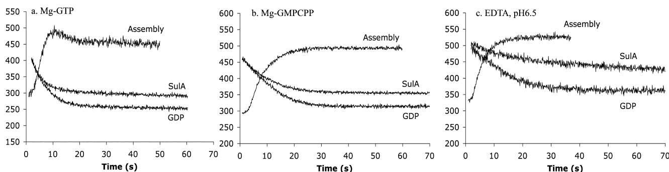
Figure 4. The assembly and disassembly of ATTO–FtsZ filaments induced by excess GDP or excess SulA. (a) Assembly in HMK buffer plus GTP; (b) in HMK plus GMPCPP; and (c) MEK plus GTP. The EcFtsZ concentration was 5 \mu\text{M} , SulA concentration was 10 \mu\text{M} , and GDP was 2 mM. The assembly curve shows the initial assembly induced by addition of 0.1 \mu\text{M} GTP or GMPCPP. At the end of that assembly SulA or GDP was added, and the disassembly was plotted as a decrease in fluorescence (these curves are shifted back to the zero time point, although there was a 1–2 s delay between the addition of SulA and the start of the fluorescence measurement).
