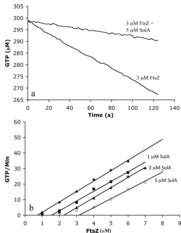
Figure 2. Inhibition of GTPase of EcFtsZ by SulA. (a) 3 \mu M EcFtsZ hydrolyzed GTP at a rate of about 15 GTP/min, which was reduced to about 3 GTP/min after adding 5 \mu M SulA. (b) The GTPase measured at increasing concentration of EcFtsZ shows that SulA increases the apparent critical concentration.
