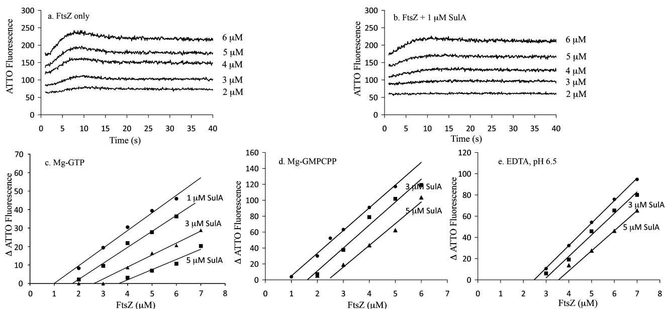
Figure 3. Assembly assayed by increase in ATTO fluorescence. EcFtsZ assembly kinetics at different concentrations of EcFtsZ without (a) and with 1 \mu M SulA (b). (c) To measure CcApp, ATTO fluorescence before adding GTP was subtracted from the fluorescence at steady state. For the curve without SulA, steady state fluorescence was averaged from 25 to 28 s, to avoid the overshoot (a). For curves with SulA the overshoot was minimal (b), and steady state was measured from 10 to 13 s. The assay was repeated for assembly in HMK plus GMPCPP (d) and in MEK buffer plus GTP (e).
