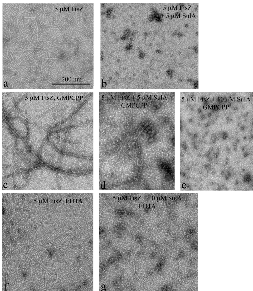
Figure 1. EM images of EcFtsZ without Sula and with the indicated addition of Sula. (a, b) In HMK buffer with GTP; (c, d, e) in HMK with GMPCPP; and (f, g) in MEK buffer with GTP.
