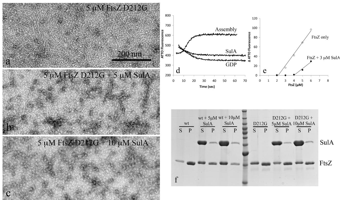
Figure 8. SulA inhibits assembly of EcFtsZ D212G. EM images of 5 \mu\text{M} Ec FtsZ D212G in HMK buffer with 1 mM GTP (a) and mixed with 5 \mu\text{M} (b) or 10 \mu\text{M} (c) SulA. Scale bar: 200 nm. Assembly and disassembly of 4.5 \mu\text{M} Ec D212G plus 0.5 \mu\text{M} ATTO–FtsZ (d). Assembly was initiated by the addition of 100 \mu\text{M} GTP. Disassembly was induced with either 2 mM GDP or 10 \mu\text{M} SulA. (e) The critical concentration of Ec FtsZ D212G was assayed by measuring the increase in ATTO fluorescence, using a 9:1 mix of D212G:ATTO–FtsZ. (f) SulA inhibition of assembly in DEAE dextran.
