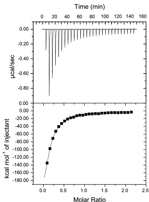
Figure 5. The binding of EcFtsZ and SulA measured by ITC. See Experimental Procedures for details of the assay. The curve fit gives the K_A as 1.29 \mu\text{M}^{-1} ( K_D = 0.78 \mu\text{M} ). For this measurement, the proteins were in HMK buffer with no GTP.
