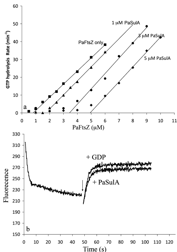
Figure 7. (a) GTPase of PaFtsZ is inhibited by SulA, primarily as an increase in the apparent critical concentration. (b) Assembly of 5 μM PaFtsZ assayed by FRET. Assembly results in a drop in donor fluorescence. Upon addition of SulA or GDP, there was a small drop in fluorescence due to the ~10% dilution, and then the donor fluorescence increased, indicating disassembly. The rate of disassembly is the same for GDP and SulA.
