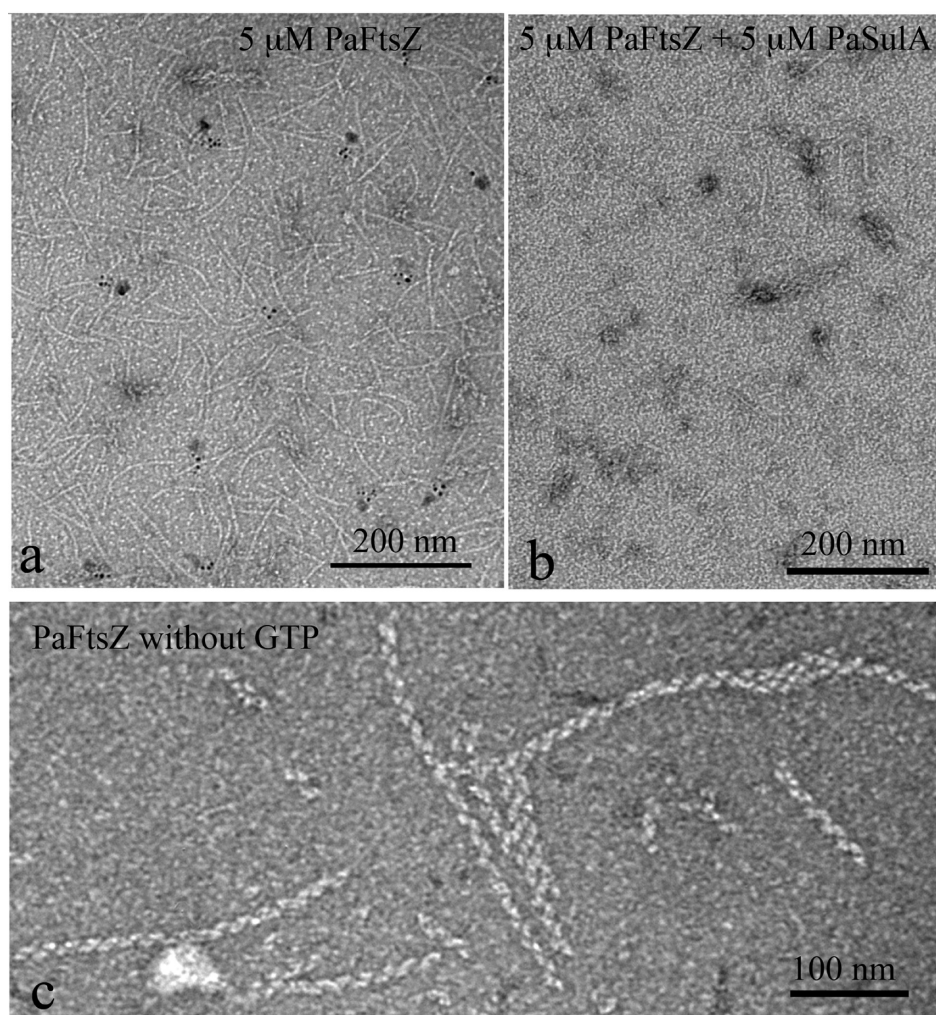
Figure 6. EM images of PaFtsZ and the inhibition of assembly by Sula. (a) 5 \mu M PaFtsZ assembled into one-stranded protofilaments in GTP. (b) After adding 5 \mu M Sula, most filaments disappeared. (c) A new polymer structure was found for PaFtsZ without added nucleotide (or in the presence of GDP). The \sim 15 nm diameter is smaller than the 23 nm diameter of EcFtsZ minirings and DEAE dextran tubes.
